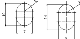
Mounting Hole
